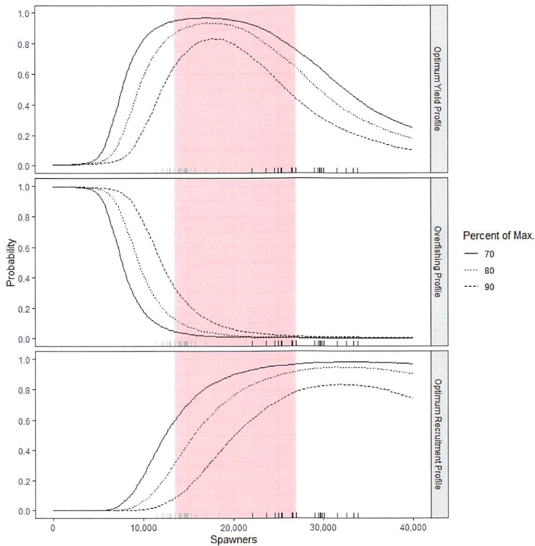
Figure 14.- Optimal yield profiles (OYP) plots for Kenai River late-run Chinook salmon 75 cm METF and longer. OYPs show probability that a specified spawning abundance will result in specified fractions (70%, 80%, and 90% line) of maximum sustained yield. Shaded areas bracket the recommended goal ranges; grey and black marks along the x-axis show comparable lower and upper bounds for other Alaskan Chinook salmon stocks scaled by S_{MSY} ratios (see Methods).
